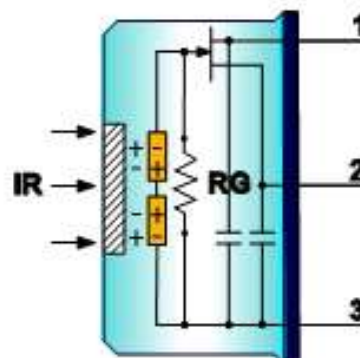
DUAL ELEMENT PYROELECTRIC INFRARED SENSOR
